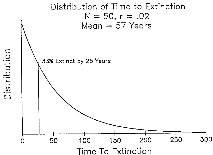
Figure 13. Exponentially distributed persistence time for a population of 50 animals growing at an exponential rate of .02 with a variation in growth rate of 0.2. While the mean (expected) persistence time is 57 years, the exponential characteristic of the distribution shows that there is a high probability of extinction before this period (33% chance by 25 years).
